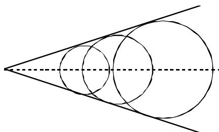
Figure 3. Circles touching two lines
